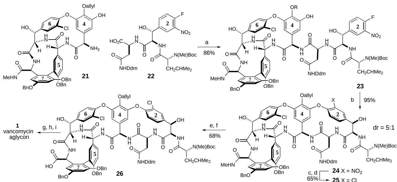
Scheme 3. Assemblage of the vancomycin aglycon. a) EDCI, HOAt, THF, 0°C; b) CsF, DMSO, room temperature; c) Zn 0 , HOAc, EtOH, 40°C; d) HBF 4 , t BuONO, MeCN, then CuCl, CuCl 2 , H 2 O; e) N 2 O 4 , NaOAc, CH 2 Cl 2 /CH 3 CN, 0°C; f) H 2 O 2 , LiOH, THF/H 2 O; g) [Pd(PPh 3 ) 4 ], morpholine, THF; h) 10% Pd/C, 1,4-cyclohexadiene, EtOH, room temperature; i) TFA, DMS, CH 2 Cl 2 , 0°C to room temperature. See ref. [6] for abbreviations.
